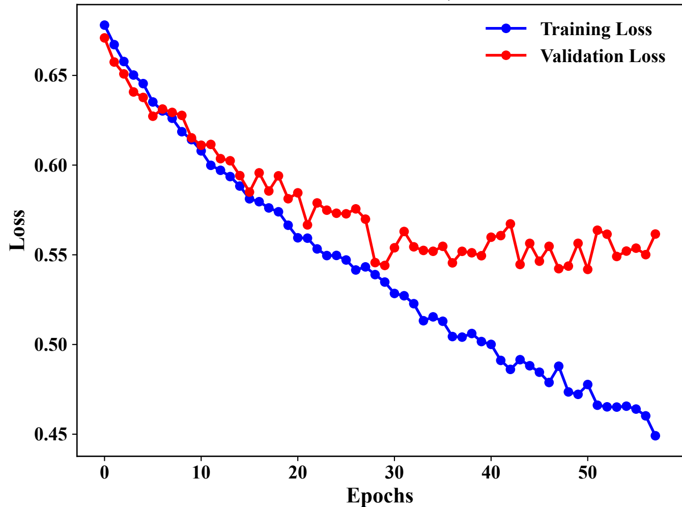
Loss Curves: Seed 24, Rank 3
